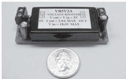
VB5V2A Voltage Booster
